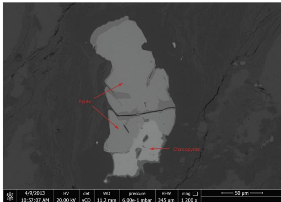
Figure 9. Irregular composite grain of Pyrite and chalcopyrite with oxidized rims (ST1).
