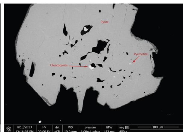
Figure 17. Composite grain of pyrite, chalcopyrite and pyrrhotite with oxidized rim (sample ST39).
