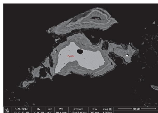
Figure 21. Oxidized pyrite in sample ST50. The difference in brightness is due to varying proportions of Fe and O.
