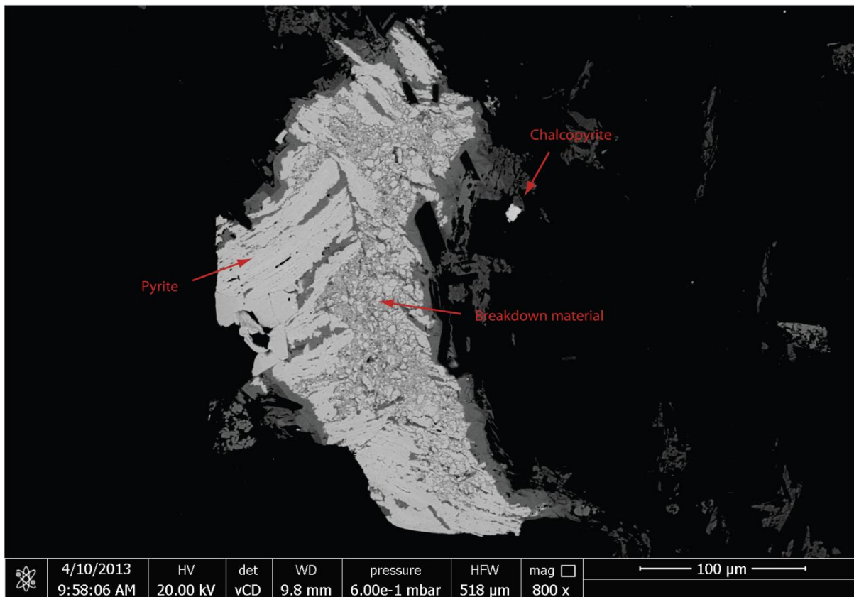
Figure 14. Composite grain of pyrite and chalcopyrite in sample ST30. Pyrite is breaking down to form mineral grains with similar chemistry to pyrite but containing trace amounts of As and Ni.
