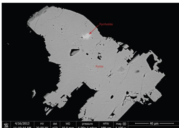
Figure 23. Same type of composite grain as in Figure 22 but with less alteration of pyrite to pyrrhotite (LL19B).
