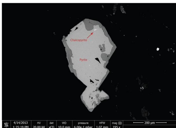
Figure 18. Composite grain of pyrite and chalcopyrite with oxidized rim in sample ST42.
